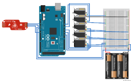
Gambar 3. Wiring Diagram Sistem
