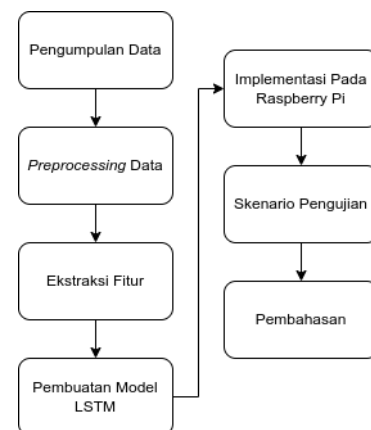
Gambar 1. Alur Penelitian
